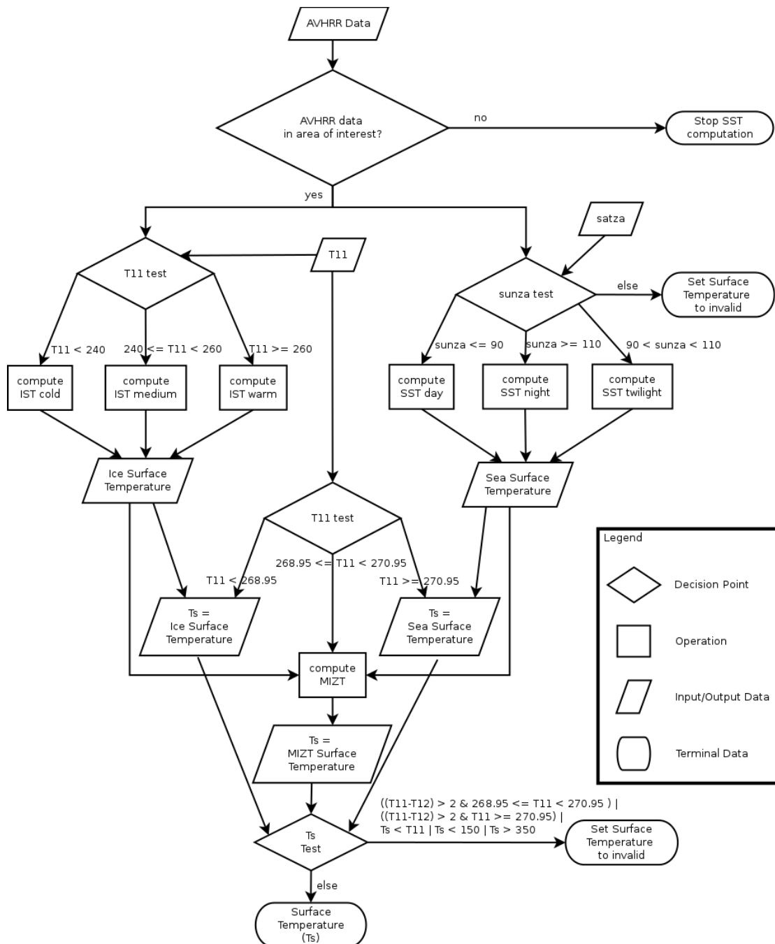
Figure 2: OSI-205 surface temperature algorithm decision tree
