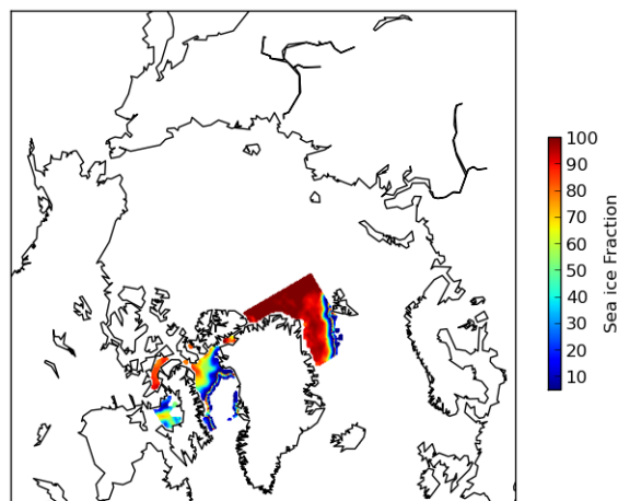
Figure 3: An ice concentration field from a 3 minute segment of a OSI-205 product.
