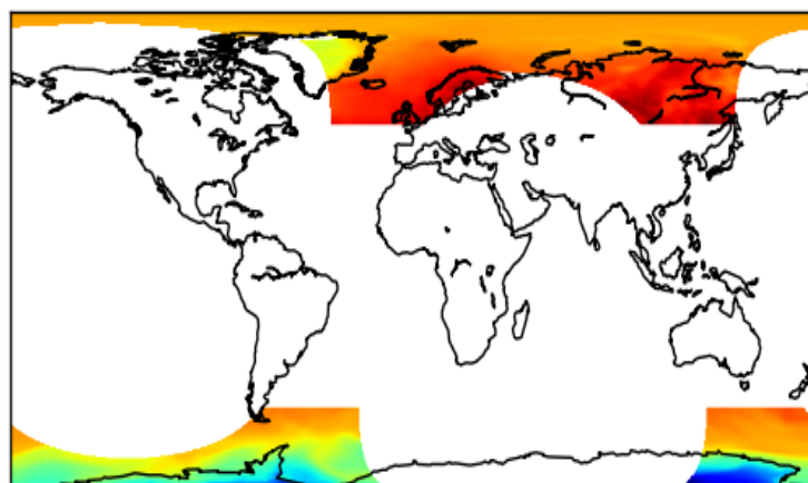
Figure 4: Product coverage is polewards of latitudes 50N and 50S. The data field is 2m Temperatures from ECMWF, corresponding to a full AVHRR swath.
