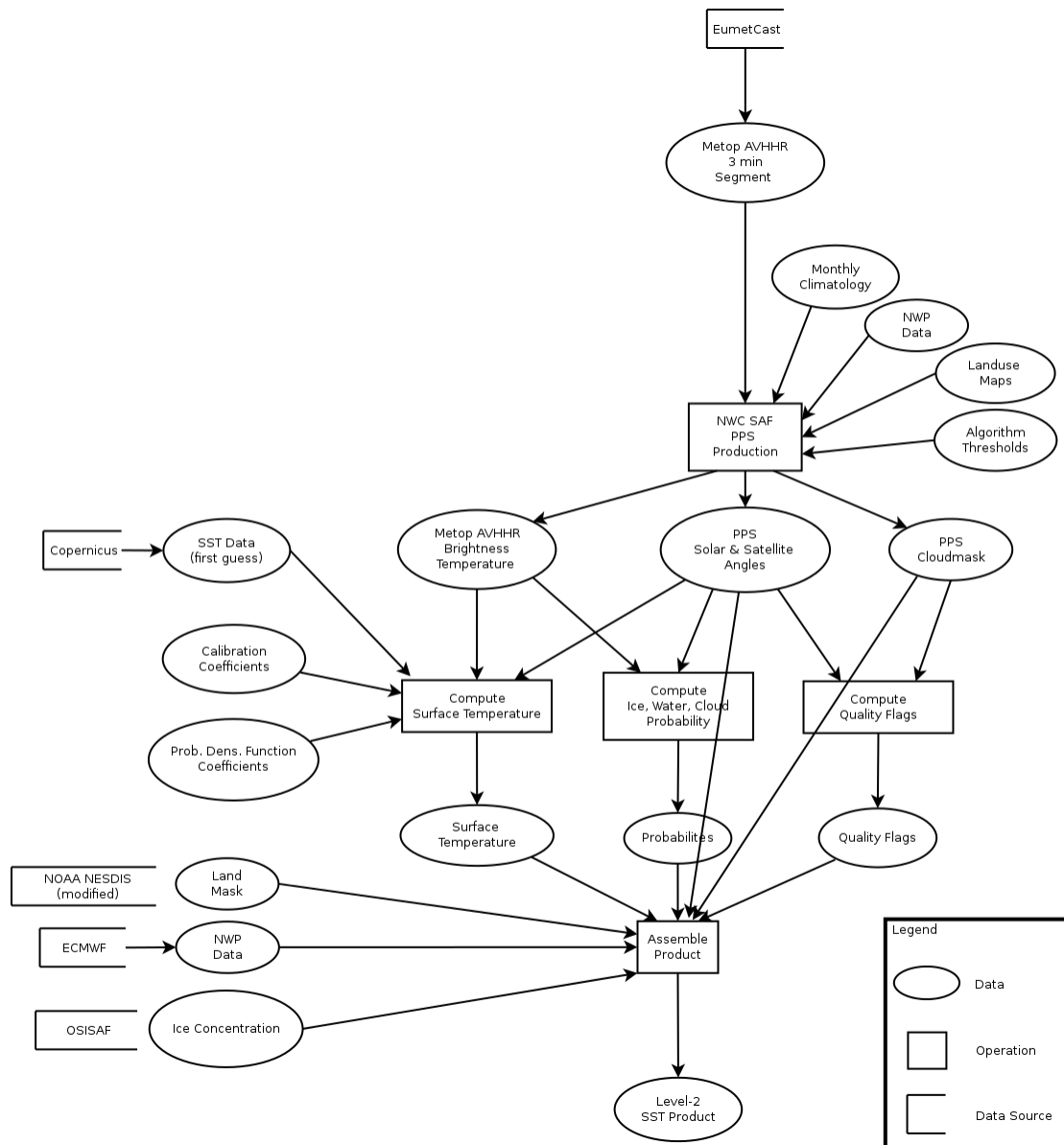
Figure 1: Overview of the Ice and Sea Surface Temperature (IST/SST) L2 processing chains (OSI-205).
