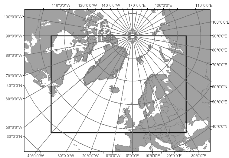
Figure 2: Coverage of the HL grid.
