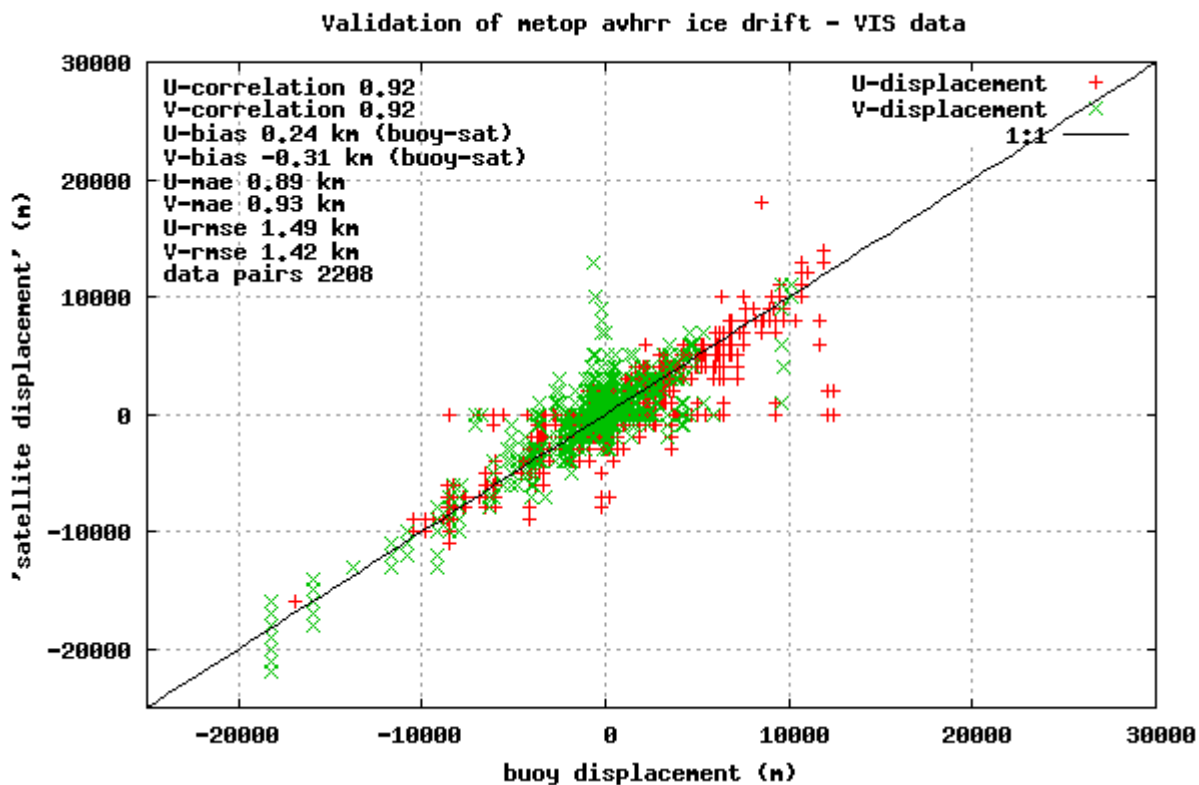
Figure 5 Scatter plot of dU_{prod} and dU_{ref} (red crosses) and dV_{prod} and dV_{ref} (green crosses), for the period 200903 to 200910. The production is based on visible data and corresponding statistics is written in table 2.
