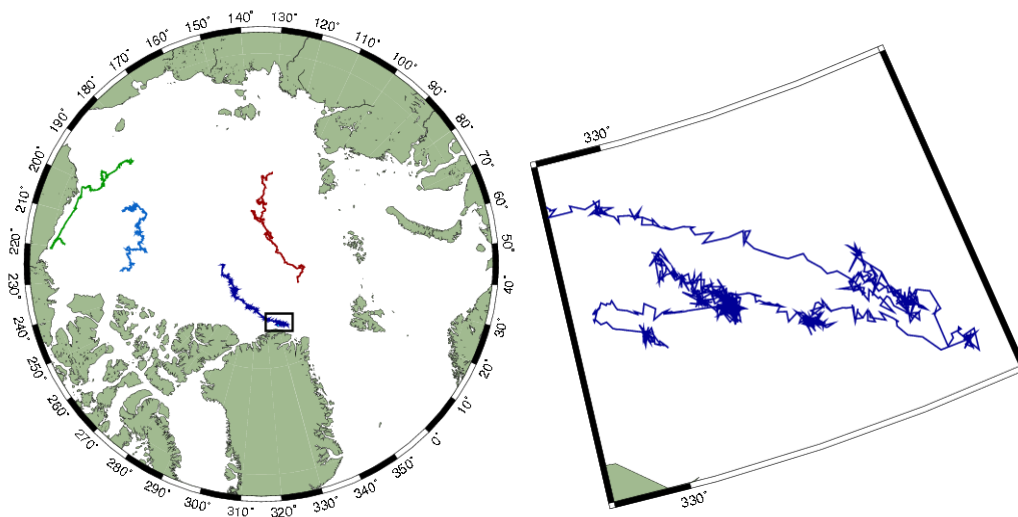
Figure 2 On the left are trajectories from 4 buoys from the validation data set during the period August 2008 to October 2009 (green – buoy48504, light blue – buoy48656, red – buoy25622 and dark blue – buoy48630). On the right is a zoom of the trajectory of buoy48630, the area indicated by black rectangle on the left.
