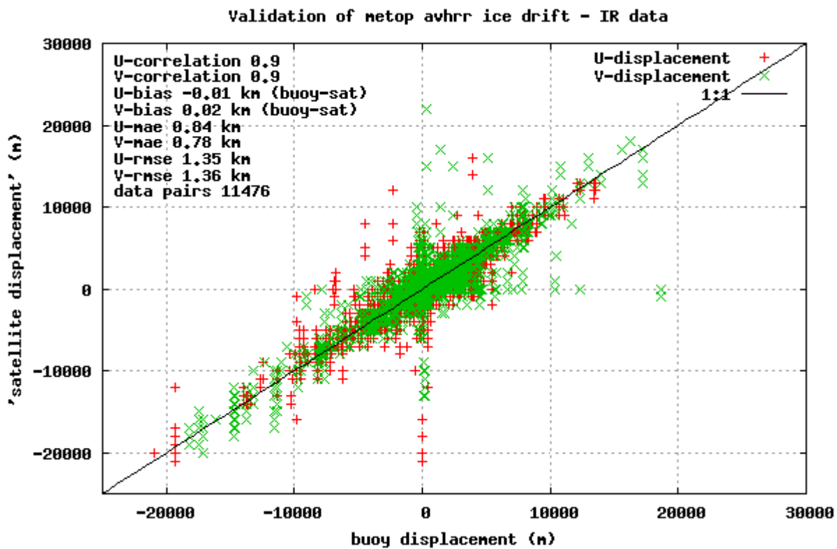
Figure 4 Scatter plot of dU_{prod} and dU_{ref} (red crosses) and dV_{prod} and dV_{ref} (green crosses), for the period 200809 to 200907. The production is based on infra red data and the corresponding statistics is written in table 1.
