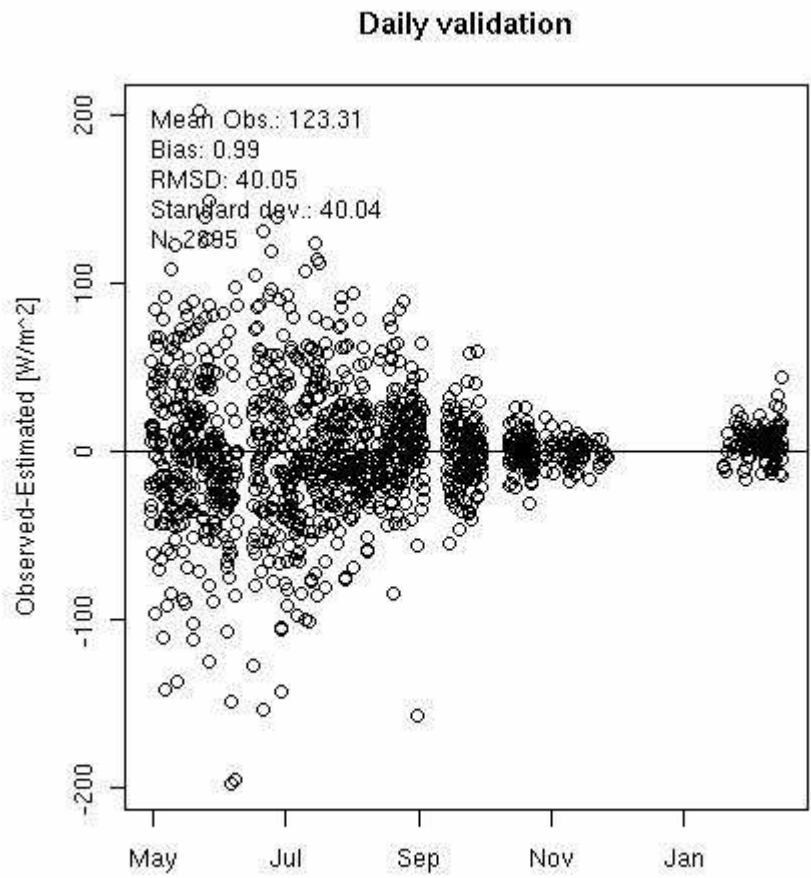
Figure 6 Quality control of daily SSI estimates against agricultural stations in Norway. The stations available for validation purposes are shown in Figure 7. All these stations measure shortwave irradiance, but only a few of them measure longwave irradiance. The validation presented above is based upon the stations on the Norwegian mainland.
