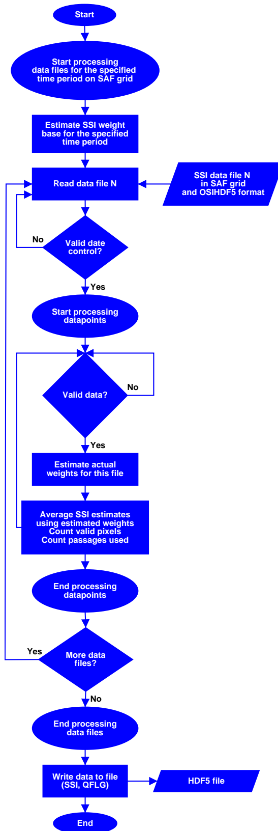
Figure 4 Processing scheme for daily estimates.
