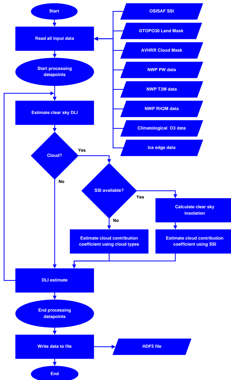
Figure 8 Instantaneous DLI estimation.
