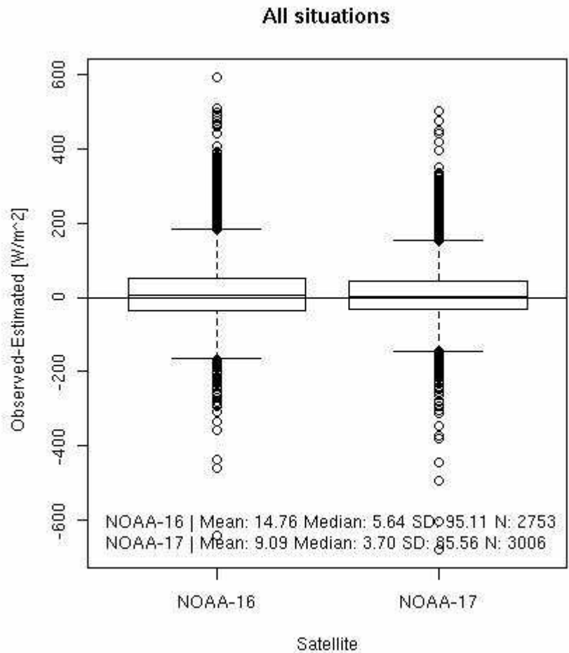
Figure 5 Quality control of instantaneous SSI estimates against agricultural stations in Norway.
