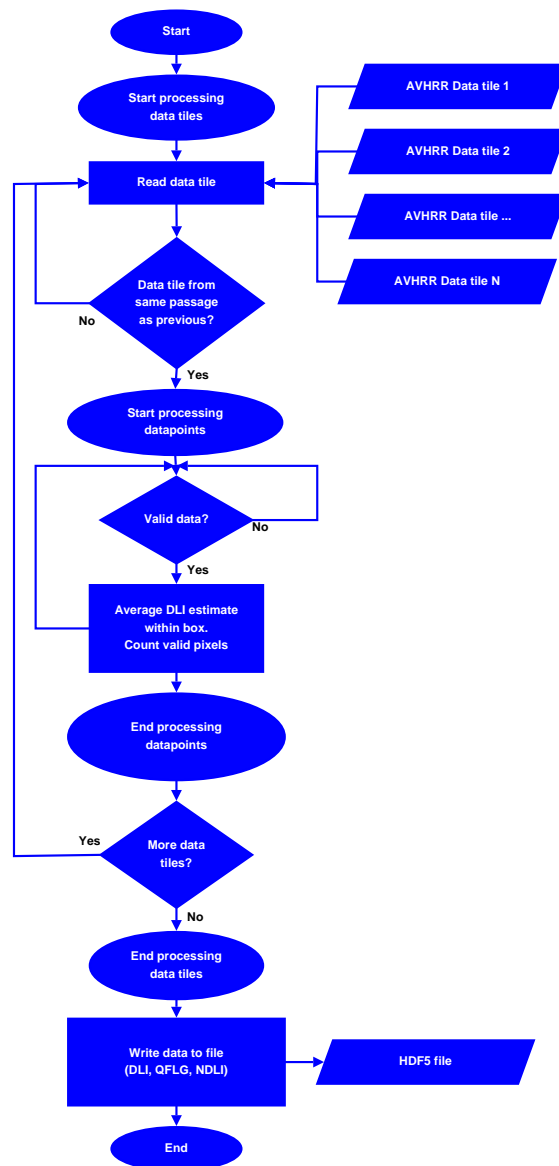
Figure 9 Processing scheme for 10 km instantaneous DLI products.
