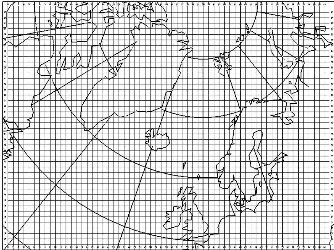
Figure 11 Area coverage of the High Latitude Ocean and sea Ice SAF SSI and DLI products with every 10'th grid point illustrated.
