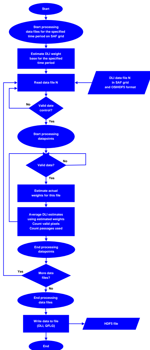
Figure 10 Processing of daily DLI estimates.
